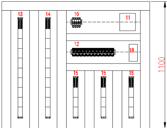
INLET VIEW
